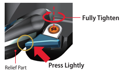
Fig.5 Fully Tighten
